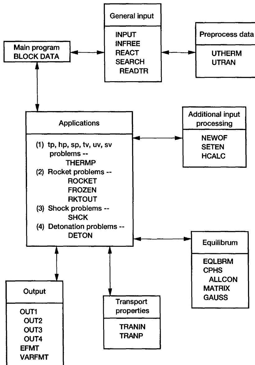
Figure 4.1.—Program modules.
