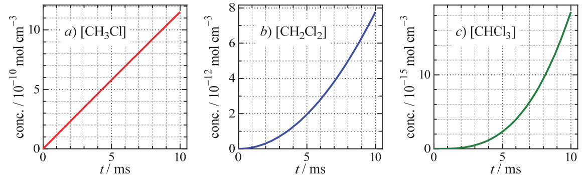
図 2.3: CH 4 -Cl 2 連鎖反応 ([CH 4 ]:[Cl 2 ]:[Ar]:[Cl] 0 = 0.01:0.04:0.95:4×10 -8 , p = 1 atm, T = 500 K).
